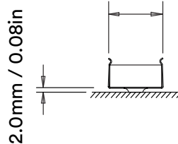
17.4mm / 0.68in
